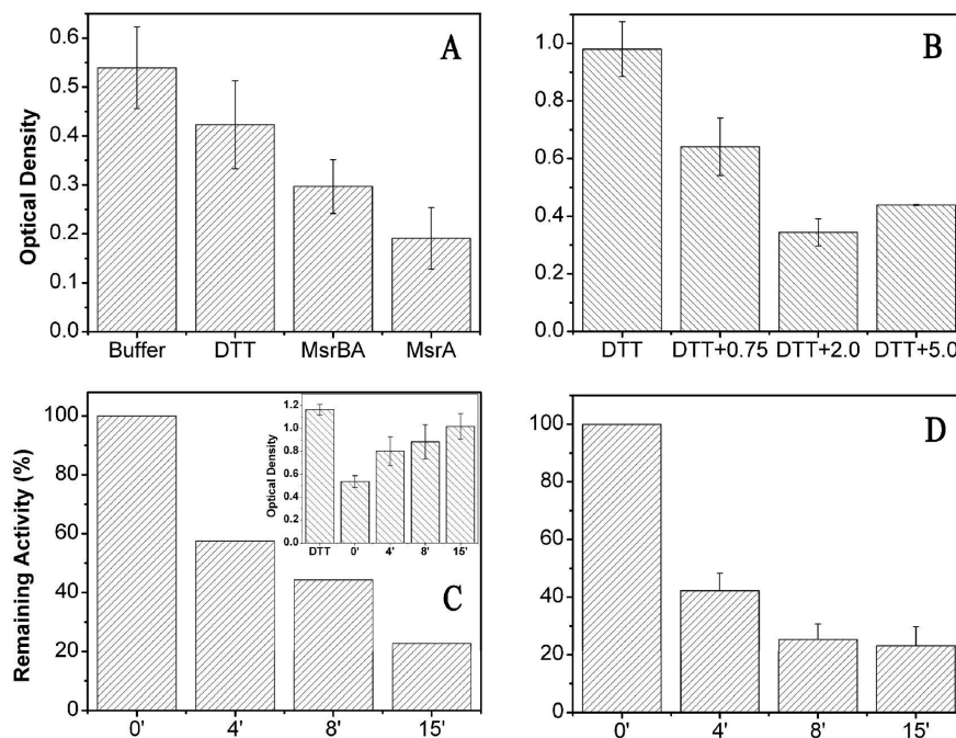
FIGURE 6: Analysis of Msr activities by ELISA using oxidized FeNos and the antibodies enriched for oxidized FeNos. (A) An EIA plate was coated with 10 \mu\text{g/mL} oxidized FeNos and then treated with 0.75 \mu\text{g} of either MsrBA or MsrA per well (in 50 \mu\text{L} ) for 1 h at room temperature. Controls included DTT treatment and addition of buffer, and blank assays included plates coated with BSA alone. After being washed, the plate was analyzed with antibodies enriched for oxidized FeNos. (B) An EIA plate was coated with 20 \mu\text{g/mL} oxidized FeNos and then treated with DTT and the indicated amount of MsrBA (in micrograms per well) for 1 h at room temperature. After being washed, the plate was assayed as described for panel A. (C and D) Analysis of the heat stability of MsrBA by an ELISA (C) and a HPLC procedure using dabsylated MetO (D). In this experiment, MsrBA (1 mg/mL) was incubated at 60 ^{\circ}\text{C} for the indicated time periods and chilled on ice, and activity remaining in the sample was assayed with an ELISA (C) and a HPLC procedure as described previously (22) (D). The inset in panel C shows changes in optical density in the ELISA following heat treatment. The left column shows absorption of the substrate treated with 2 mM DTT, and the remaining columns indicate absorption of the substrate treated with 2 mM DTT and the enzyme after heating for the indicated periods of time.
