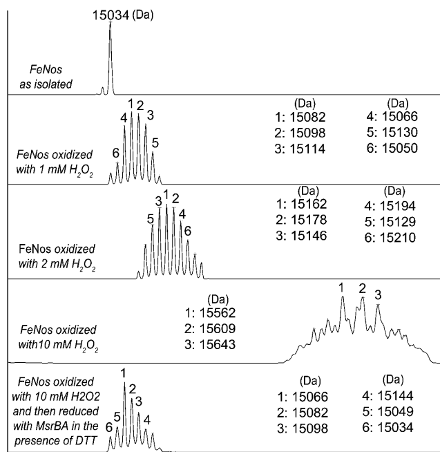
FIGURE 3: Mass spectrometry analysis of FeNos. Analysis of isolated (top panel), oxidized (three center panels), and oxidized and then reduced FeNos (bottom panel) by ESI-MS. Treatment conditions are indicated on the left side of each spectrum. Reduction reactions were conducted at 37 °C for 2 h. Major peaks are numbered, and their masses (in daltons) are shown to the right (of left) of the spectra.
