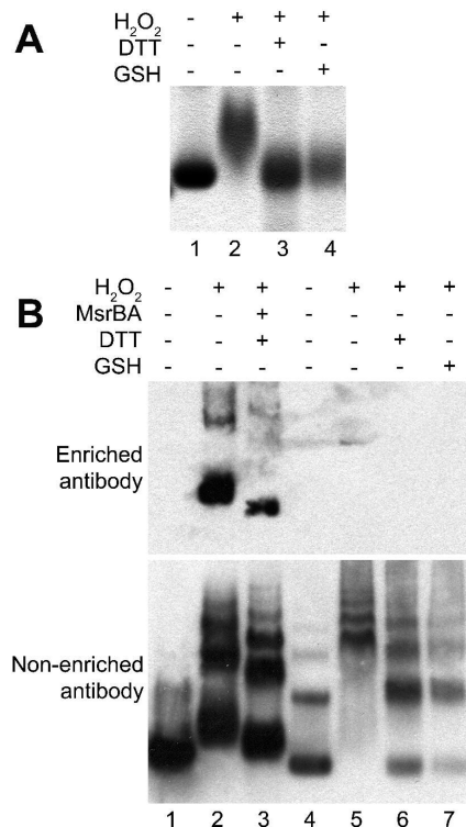
FIGURE 8: Redox properties of SeMet-FeNos. (A) SeMet-FeNos (lane 1) and SeMet-FeNos oxidized with 1 mM H 2 O 2 (lane 2) and then reduced with 5 mM DTT (lane 3) or 5 mM GSH (lane 4). (B) Immunoblot analysis of FeNos (lanes 1–3) and SeMet-FeNos (lanes 4–7) with antibodies enriched for the oxidized form of FeNos (top panel) and nonenriched antibodies (bottom panel): FeNos (lane 1), FeNos oxidized with 5 mM H 2 O 2 (lane 2) and then reduced with MsrBA in the presence of DTT (lane 3), as-isolated SeMet-FeNos (lane 4), and SeMet-FeNos oxidized with 1 mM H 2 O 2 (lane 5) and then reduced with 5 mM DTT (lane 6) or 5 mM GSH (lane 7).
