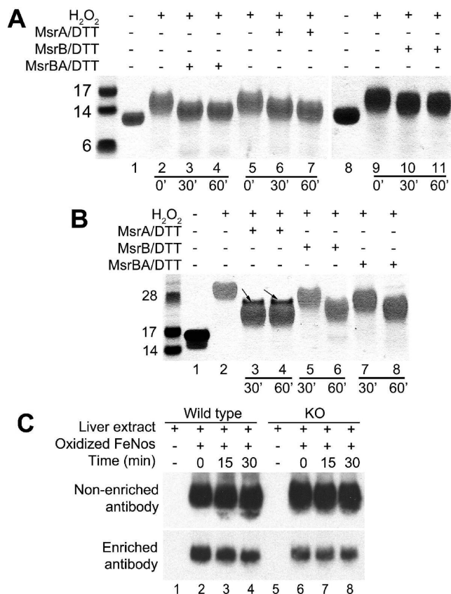
FIGURE 5: Qualitative detection of Msr activities on SDS-PAGE gels using oxidized MRPs as substrates. (A) FeNos was oxidized with 5 mM H 2 O 2 for 12 h at room temperature, dialyzed against PBS, and subjected to treatment with Msrs at a ratio of 1:20 (enzyme:substrate, w/w) for the indicated time periods. (B) LegP was oxidized with 5 mM H 2 O 2 for 12 h at room temperature, dialyzed against PBS, and treated with Msrs and DTT at a ratio of 1:20 (enzyme:substrate, w/w) for the indicated time periods. Arrows indicate the mouse MsrA used in the reduction. (C) Analysis of methionine sulfoxide reductase activity in liver extracts. Three micrograms of oxidized FeNos were incubated with 15 \mu g of liver extract from wild-type (Wild type) or selenocysteine tRNA knockout (KO) mice at 37 °C for the indicated time periods. Samples were analyzed by Western blotting with antibodies enriched for oxidized FeNos (bottom panel) and with non-enriched antibodies (top panel).
