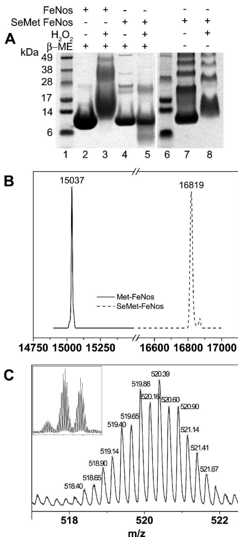
FIGURE 7: SeMet-FeNos. (A) SDS-PAGE analysis of FeNos (lanes 2 and 3) and SeMet-FeNos (lanes 4, 5, 7, and 8). FeNos was purified from cells grown in LB medium and SeMet-FeNos from cells grown in M9 minimal medium supplemented with SeMet. Lanes 1 and 6 show molecular mass standards. Other treatment conditions are indicated above lanes (SDS-PAGE sample buffer did not contain reductants). (B) Intact mass of FeNos and SeMet-FeNos determined by ESI-MS. (C) An m/z profile of a C-terminal peptide containing three SeMet residues. Masses of quadruply charged ions are shown above peaks and correspond to a complex selenium isotopic distribution from three Se atoms. The inset shows a profile of three ions with oxidation of one, two, or three SeMet residues. Each of these three broad peaks is composed of narrow peaks due to Se isotope distribution. Panel C shows the peak at the center of the inset, in which two SeMet residues were oxidized.
