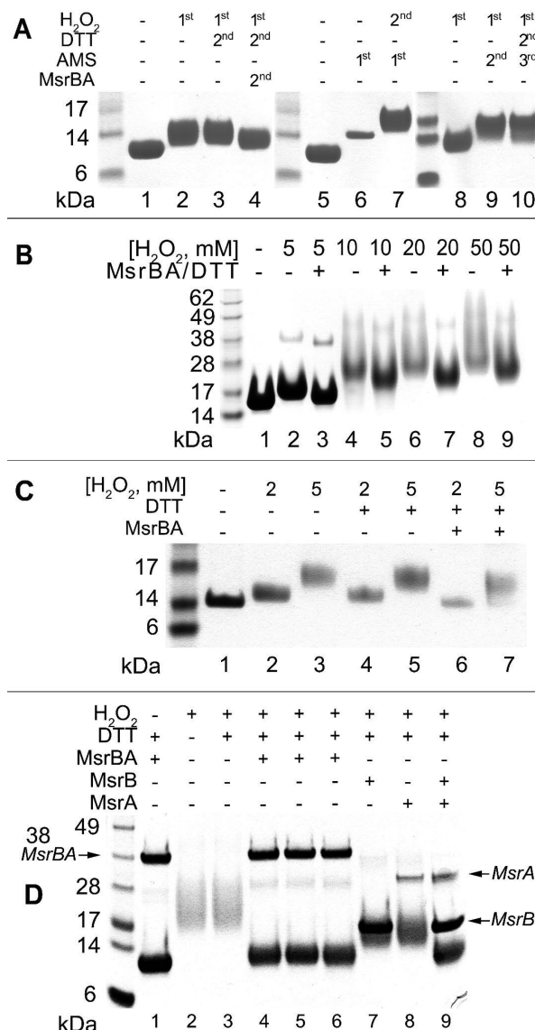
FIGURE 2: Mobility of oxidized and reduced MRPs on SDS-PAGE gels. Proteins were electrophoresed on 10% SDS-PAGE gels and stained with Coomassie blue. Lanes with protein standards are not numbered. (A) FeNos as isolated (lanes 1 and 5), FeNos oxidized with 5 mM H 2 O 2 at pH 5.0 for 12 h (lanes 2 and 8), DTT-treated oxidized FeNos (lane 3), oxidized FeNos further treated with MsrBA for 2 h [lane 4; unless otherwise noted, all treatments with enzymes were at a 1:20 (w/w) enzyme:substrate ratio, at 37 °C for 2 h], AMS-alkylated FeNos (lane 6), oxidized alkylated FeNos (lane 7), FeNos oxidized after alkylation (lane 9), and oxidized FeNos treated with DTT and then alkylated (lane 10). (B) LegP (lane 1), LegP with the indicated H 2 O 2 concentrations (lanes 2, 4, 6, and 8), and oxidized LegP treated with MsrBA in the presence of 20 mM DTT (lanes 3, 5, 7, and 9). (C) CTR1-N (lane 1), CTR1-N oxidized with the indicated concentrations of H 2 O 2 (lanes 2 and 3) and then treated with 20 mM DTT (lanes 4 and 5) or MsrBA and 20 mM DTT (lanes 6 and 7). (D) FeNos treated with MsrBA and DTT (lane 1), FeNos oxidized with 10 mM H 2 O 2 at pH 7.0 (lane 2) for 12 h, H 2 O 2 removed by dialysis, and the protein treated for 2 h at 37 °C with 20 mM DTT (lane 3), 4 \mu M MsrBA and 20 mM DTT (lanes 4–6), 4 \mu M MsrB and 20 mM DTT (lane 7), 1 \mu M MsrA and 20 mM DTT (lane 8), or both enzymes and 20 mM DTT (lane 9). Migration of MsrA, MsrB, and MsrBA is indicated by arrows. The other major lower band (see lanes 1, 4–6, and 9) is the reduced FeNos. Upon oxidation (lane 2 and 3) or oxidation following a partial reduction (lanes 7 and 8), this protein migrates more slowly.
