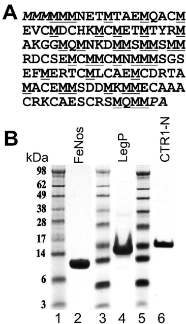
FIGURE 1: Methionine-rich proteins (MRPs). (A) Amino acid sequence of FeNos, an MRP from Nostoc sp. Methionine (M) residues are underlined. Residues shown in italics were encoded in the FeNos gene, but were not included in the expression construct. (B) SDS–PAGE analysis of protein markers (lanes 1, 3, and 5) and purified recombinant FeNos (lane 2), LegP (lane 4), and CTR1-N (lane 6). Note that the 15 kDa FeNos migrates as a 10 kDa protein. Proteins were electrophoresed on a 10% SDS–PAGE gel and stained with Coomassie blue.
