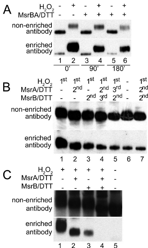
FIGURE 4: Western blot analyses of MRPs with antibodies enriched for their oxidized forms. (A) FeNos was analyzed with antibodies enriched for oxidized FeNos (bottom panel) and with non-enriched antibodies (top panel). The time of reduction (in minutes) is indicated below the panel. (B) FeNos was analyzed with antibodies against oxidized FeNos (bottom panel) and with non-enriched antibodies (top panel). 1st, 2nd, and 3rd indicate the order in which the corresponding treatments were made. (C) LegP was analyzed with antibodies enriched for oxidized LegP (bottom panel) or with non-enriched antibodies (top panel). Two micrograms of MRPs, either treated or not treated with H 2 O 2 and Msrs as indicated above the panels, was loaded onto each lane.
